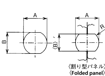
取付仕様図 / Specification drawing
