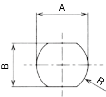
取付仕様図 / Specification drawing
