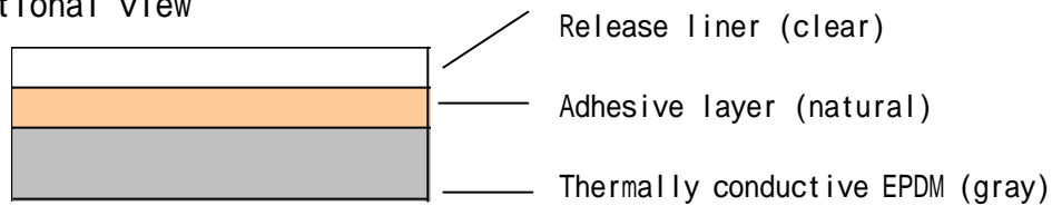
Cross-sectional view
